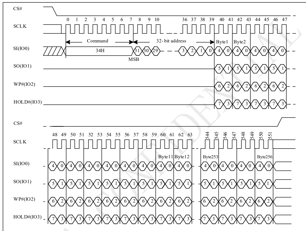
Figure 10-46 Quad Page Program with 4-Byte Address Sequence (SPI)
