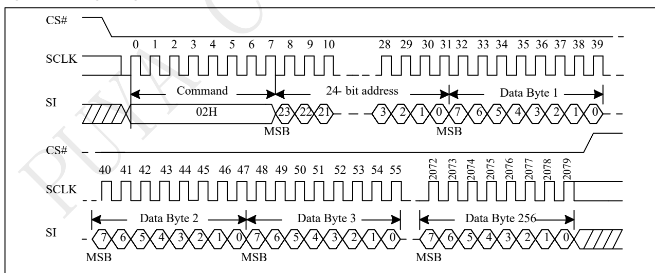
Figure 10-43 Page Program (PP) Sequence (SPI)
