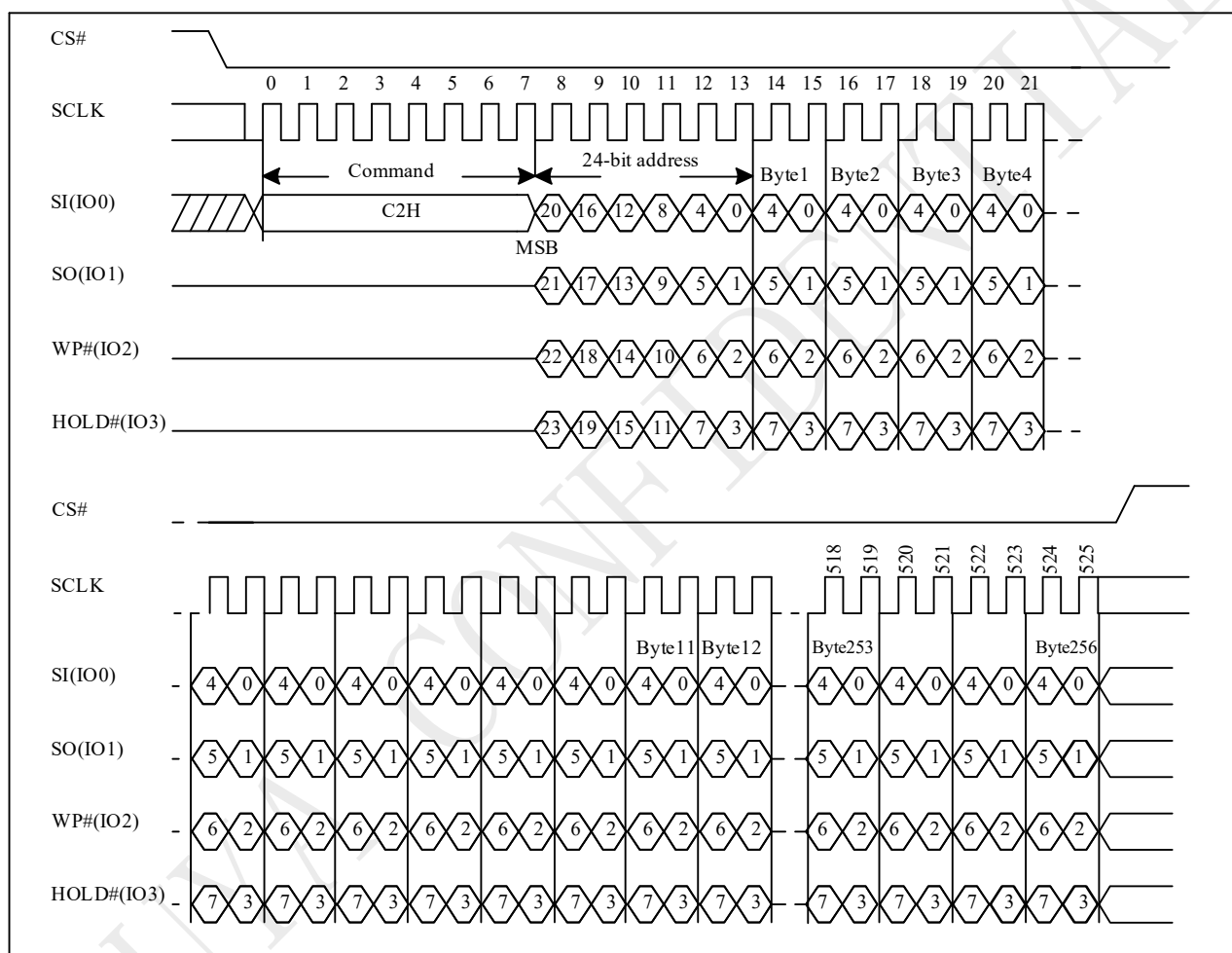
Figure 10-47 Quad Page Program (QPP) Sequence (SPI)
