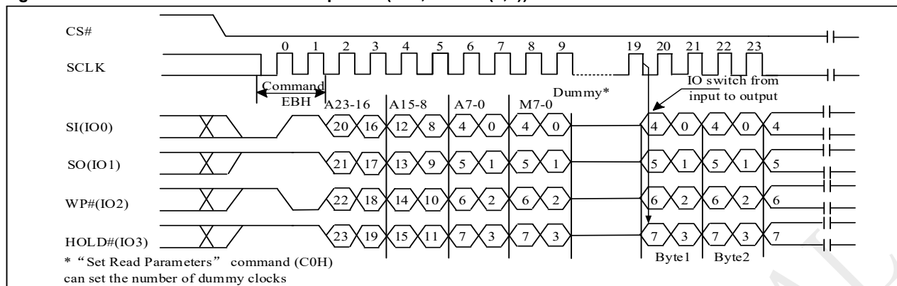
Figure 10-25a 4IO Read in QPI mode Sequence (QPI, M5-4 ≠ (1,0))
