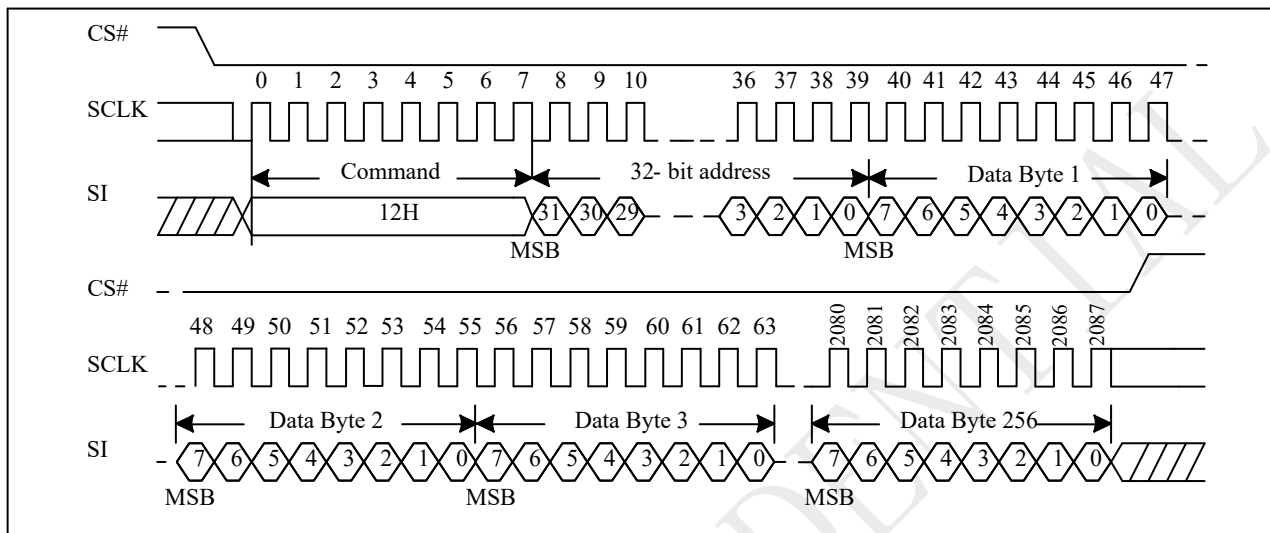
Figure 10-44 Page Program with 4-Byte Address Sequence (SPI)
