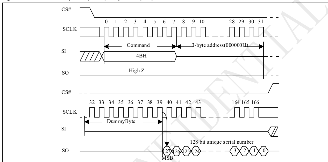
Figure 10-69 Read Unique ID (RUID) Sequence (SPI)
