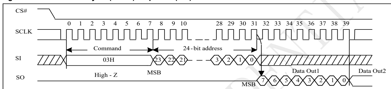
Figure 10-13 Read Data Bytes (READ) Sequence (SPI)
