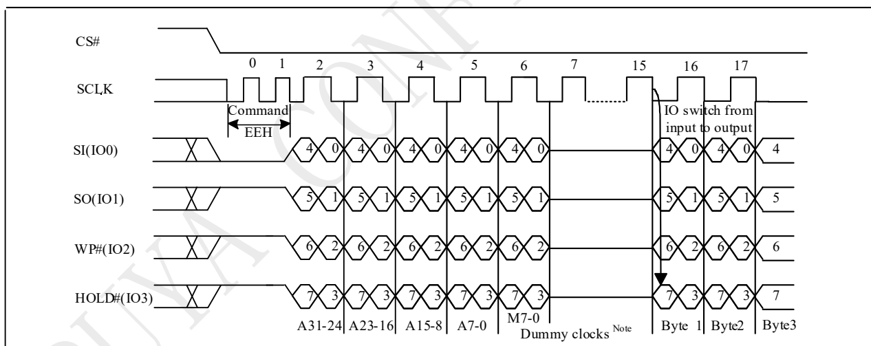
Figure 10-28a DTR 4IO Read with 4-Byte Address Sequence (QPI, M5-4 ≠ (1,0))
