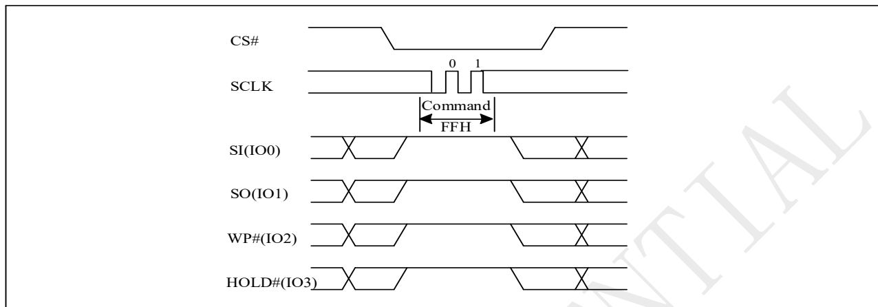
Figure 10-35 Disable QPI Sequence (QPI)
