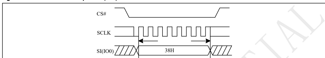
Figure 10-34 Enable QPI Sequence (SPI)
