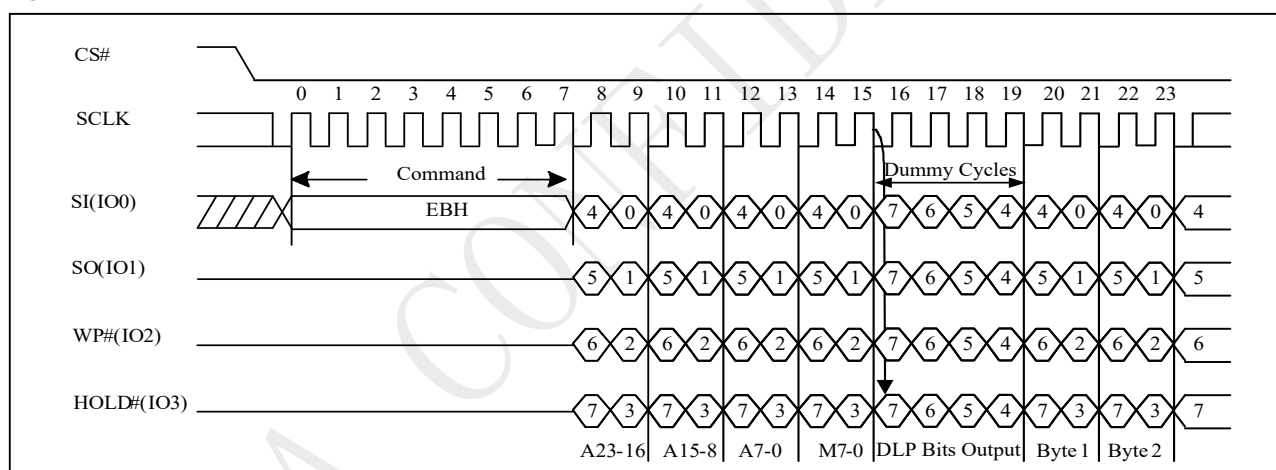
Figure 10-33e 4IO Read with DLP bits output Sequence (SPI)
