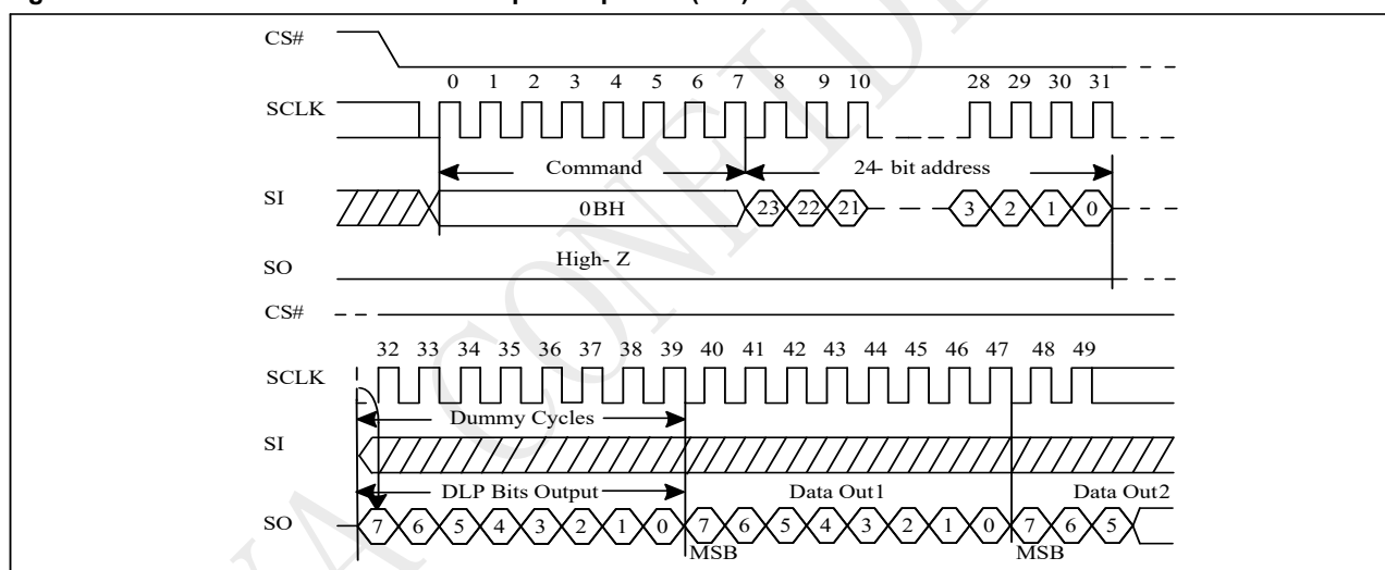
Figure 10-33 Fast Read with DLP bits output Sequence (SPI)
