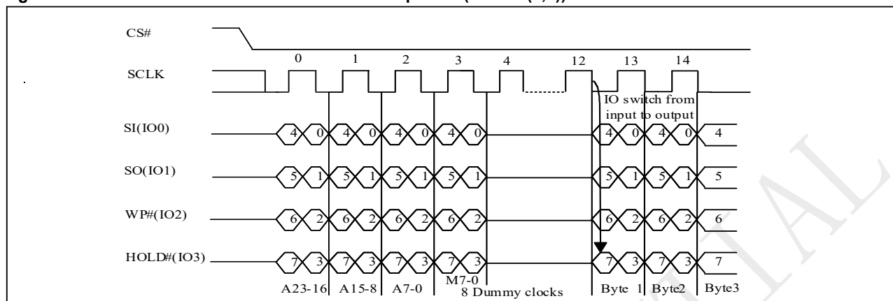
Figure 10-27a DTR 4IO Continuous Read Mode Sequence (M5-4 = (1,0))
