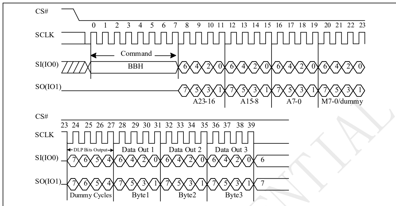
Figure 10-33d 2IO Read with DLP bits output Sequence (SPI)
