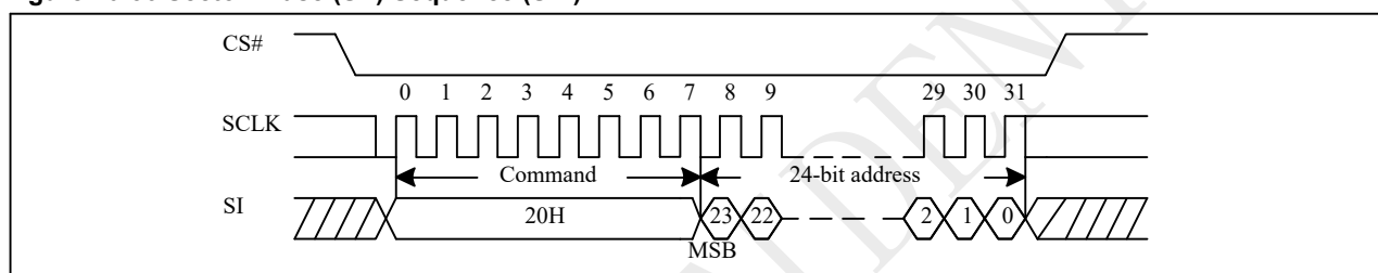
Figure 10-36 Sector Erase (SE) Sequence (SPI)
