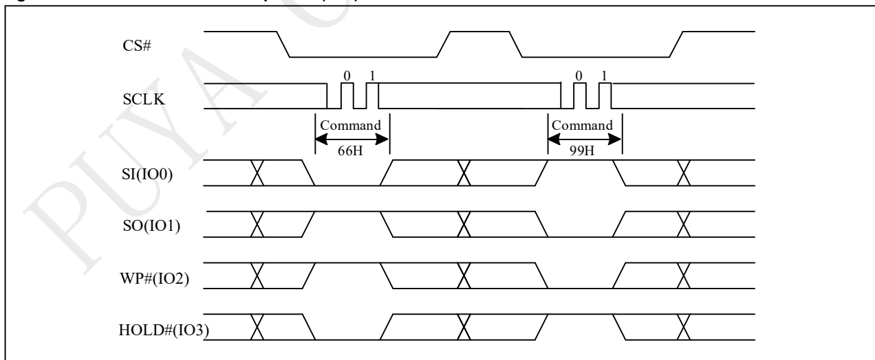
Figure 10-66b Software Reset Sequence (QPI)
