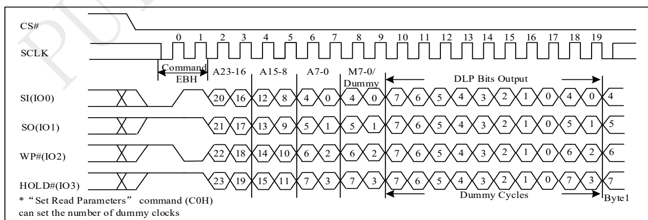
Figure 10-33f 4IO Read with DLP bits output Sequence (QPI)
