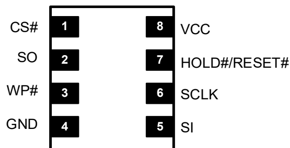
8-Pad WSON (8x6mm)
