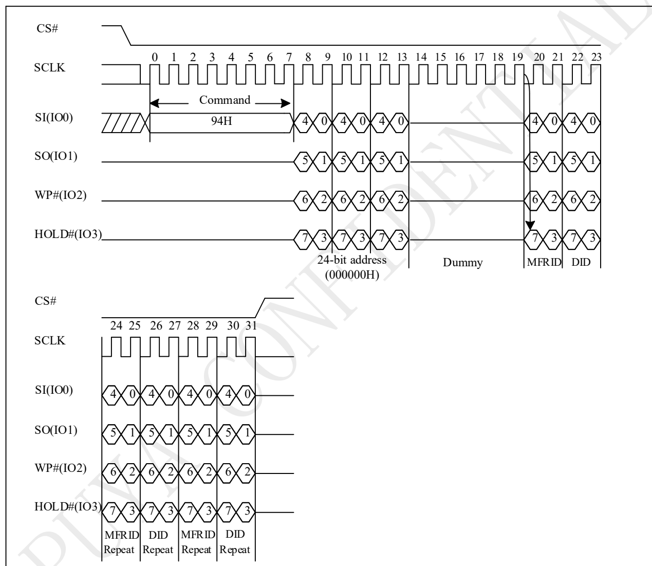
Figure 10-56 QUAD I/O Read Electronic Manufacturer & Device ID (QREMS) Sequence (SPI)
