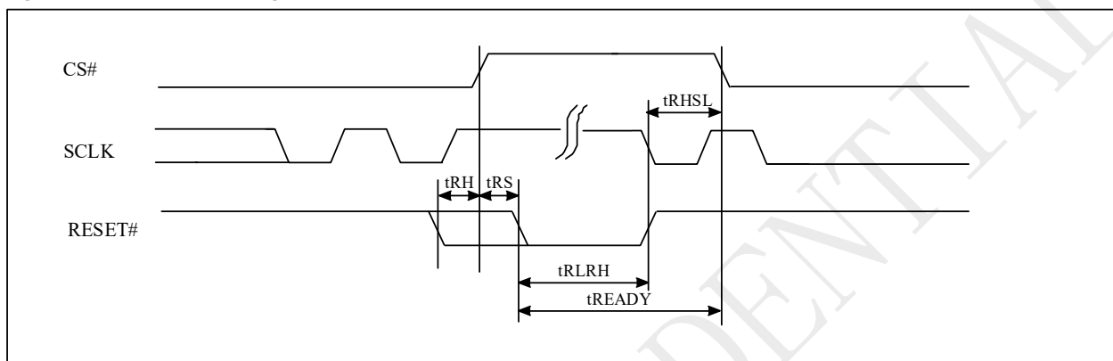
Figure 10-67 RESET Timing
