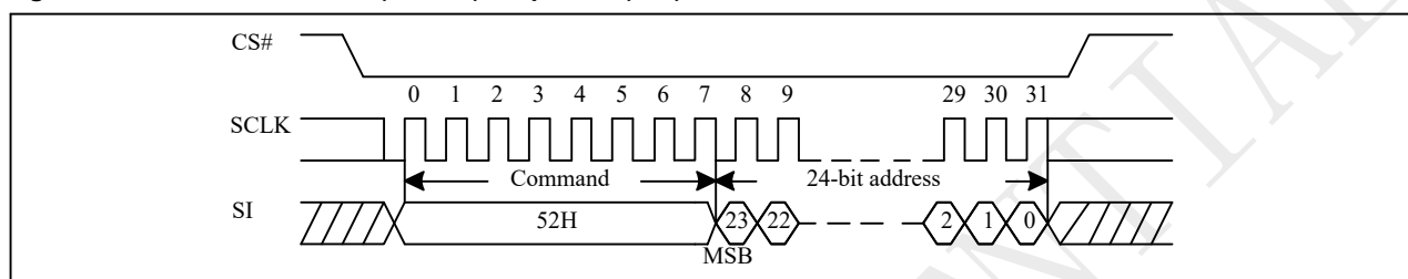
Figure 10-38 Block Erase 32K(BE32K) Sequence (SPI)
