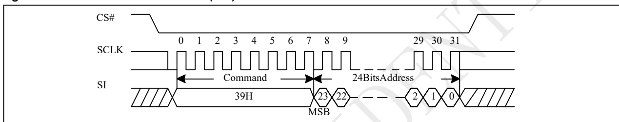
Figure 10-62 Individual Block Unlock (SPI)
