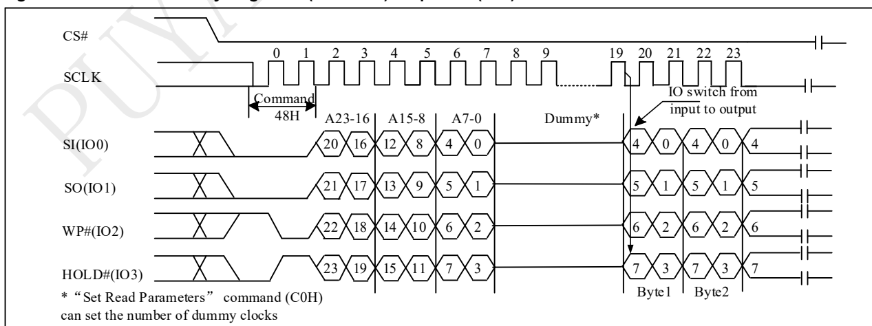
Figure 10-51a Read Security Registers (RDSCUR) Sequence (QPI)
