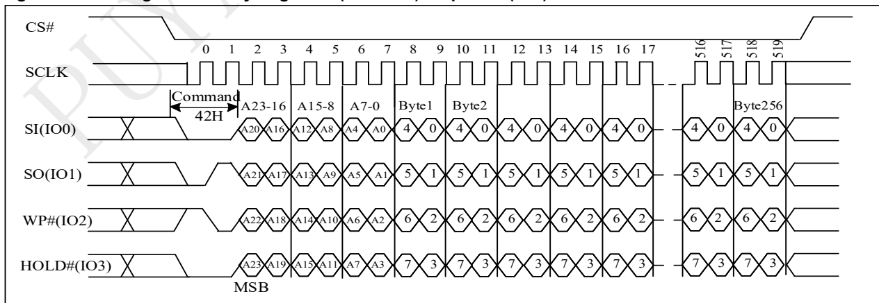
Figure 10-50a Program Security Registers (PRSCUR) Sequence (QPI)
