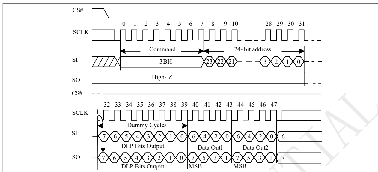
Figure 10-33b Dual Read with DLP bits output Sequence (SPI)
