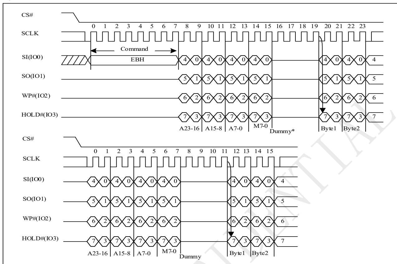
Figure 10-25b 4IO Continuous Read Sequence (SPI, M5-4 = (1,0))
