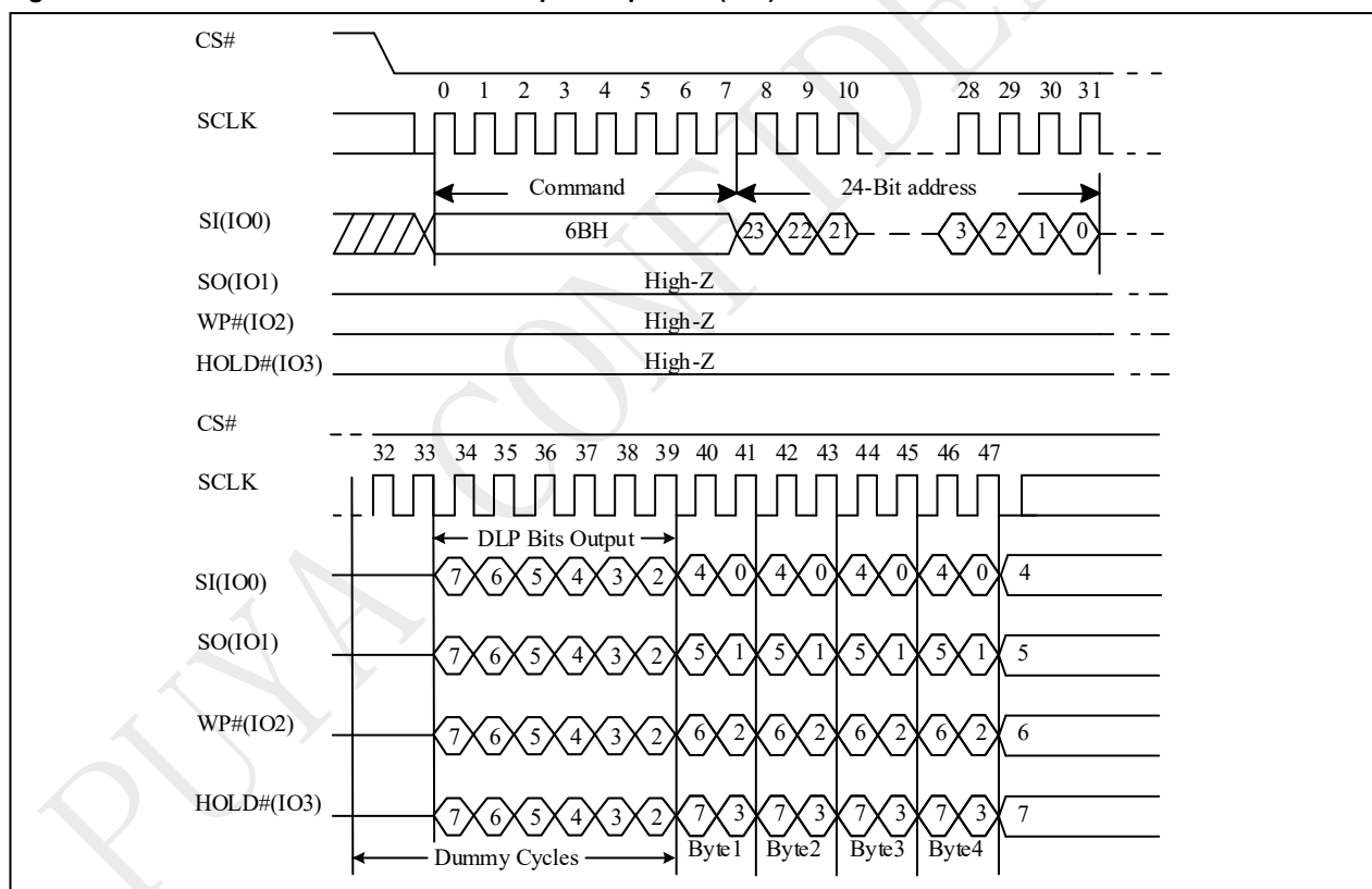
Figure 10-33c Quad Read with DLP bits output Sequence (SPI)
