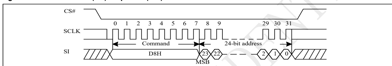
Figure 10-40 Block Erase (BE) Sequence (SPI)
