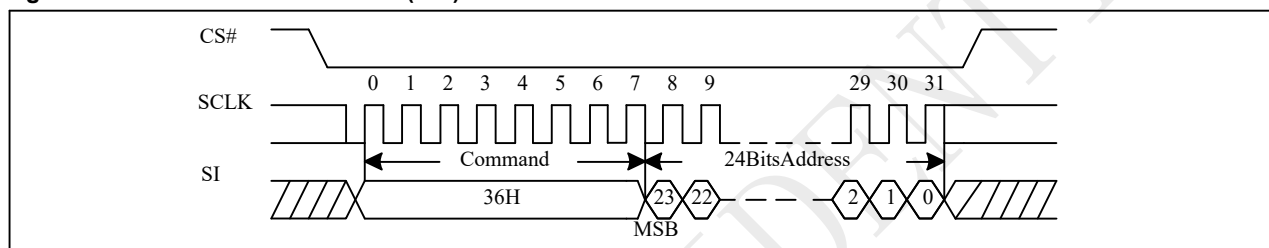
Figure 10-61 Individual Block Lock (SPI)
