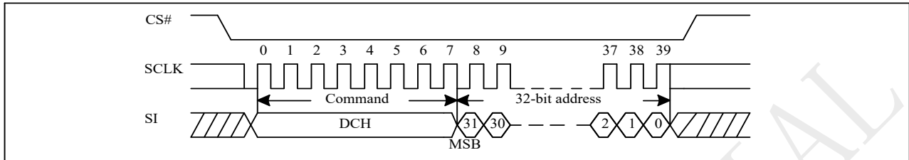
Figure 10-41 Block Erase with 4-Byte Address Sequence (SPI)
