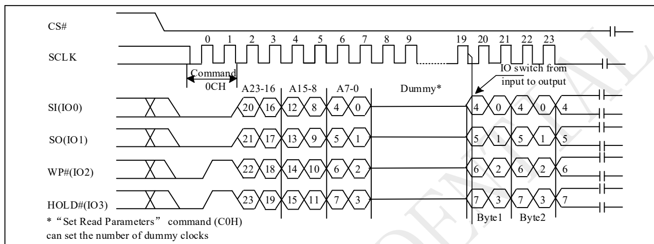
Figure 10-31 Burst Read with Wrap Sequence (QPI)
