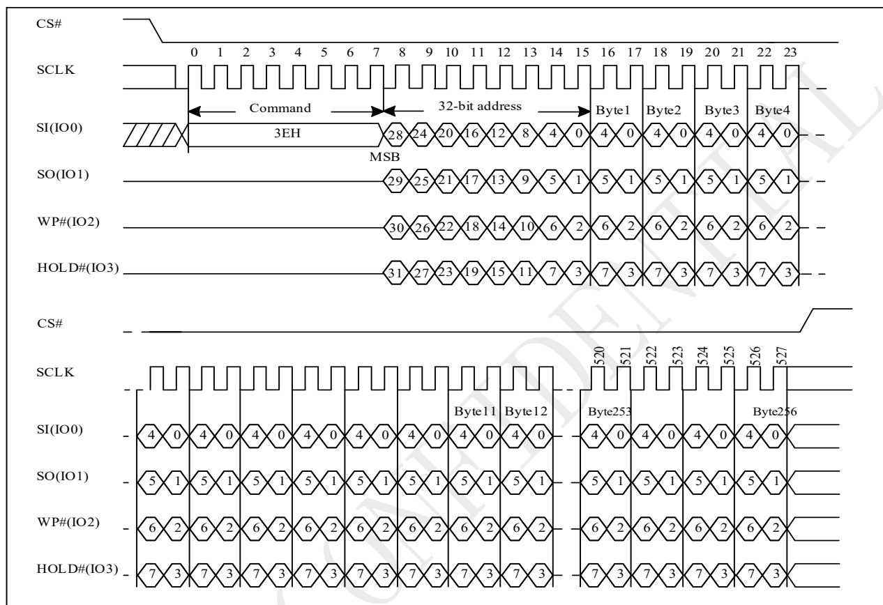
Figure 10-48 Quad-In Page Program with 4-Byte Address Sequence (SPI)
