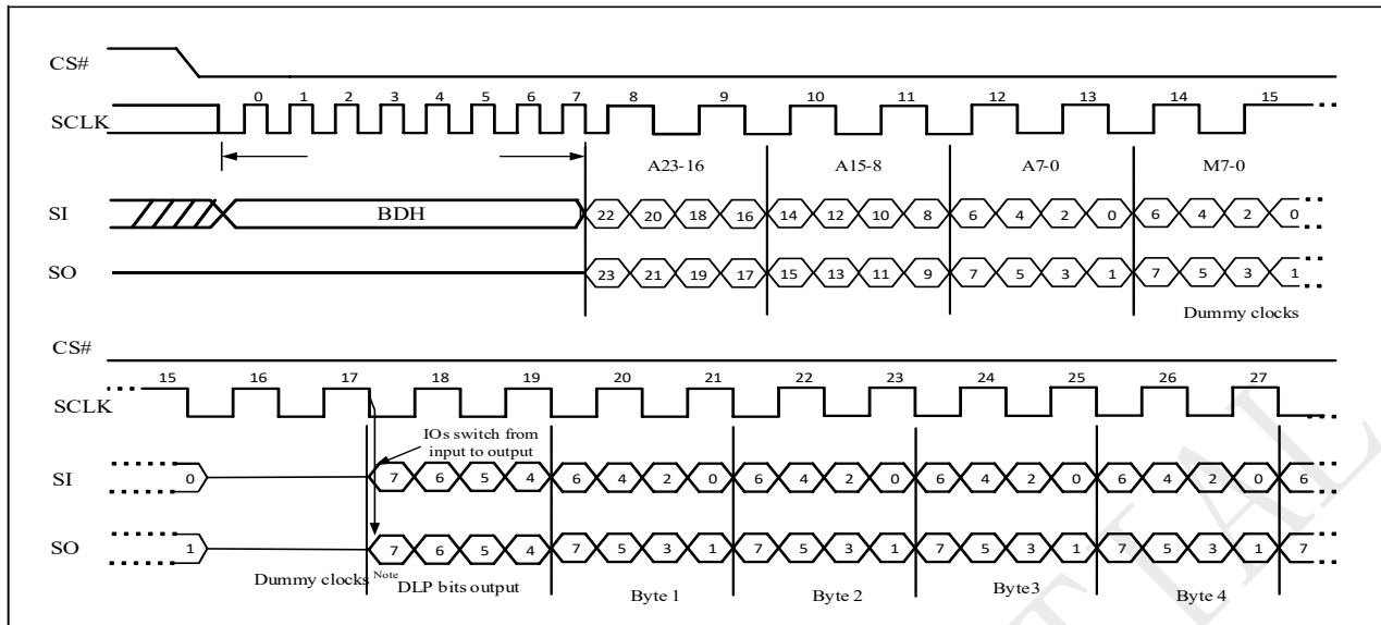
Figure 10-33j DTR 4IO Read with DLP bits output Sequence (SPI)
