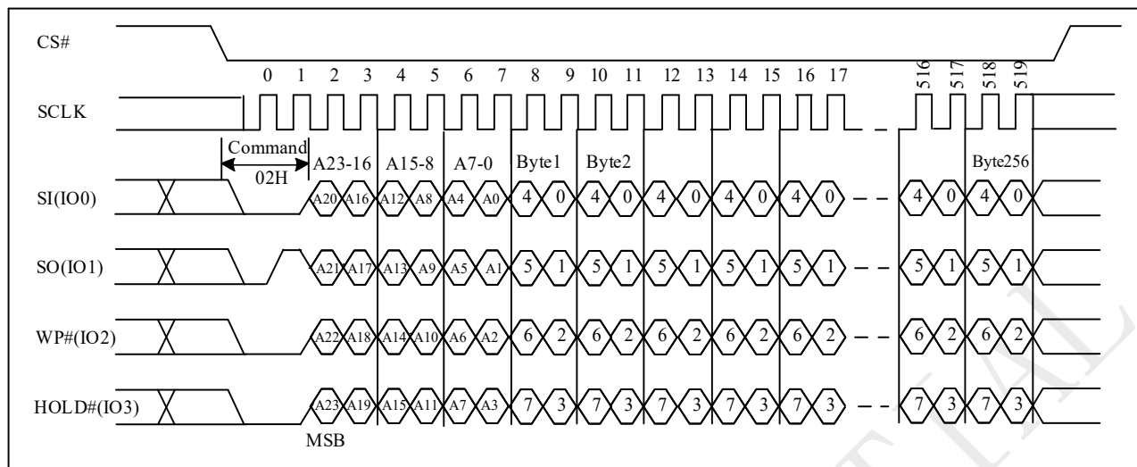
Figure 10-42a Page Program (PP) Sequence (QPI)
