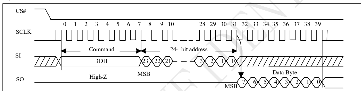
Figure 10-63 Read Block Lock Status (SPI)
