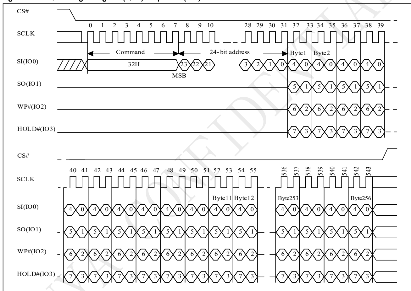
Figure 10-45 Quad Page Program (QPP) Sequence (SPI)
