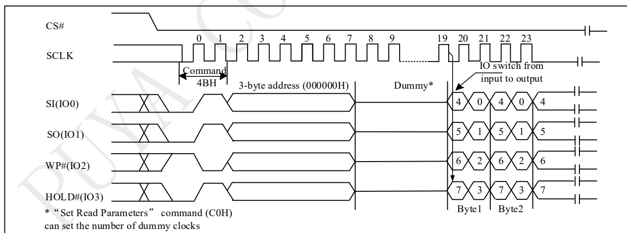
Figure 10-69a Read Unique ID (RUID) Sequence (QPI)
