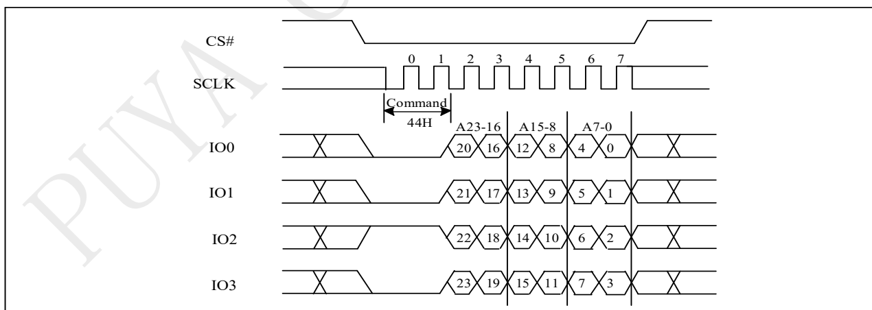
Figure 10-49a Erase Security Registers (ERSCUR) Sequence (QPI)
