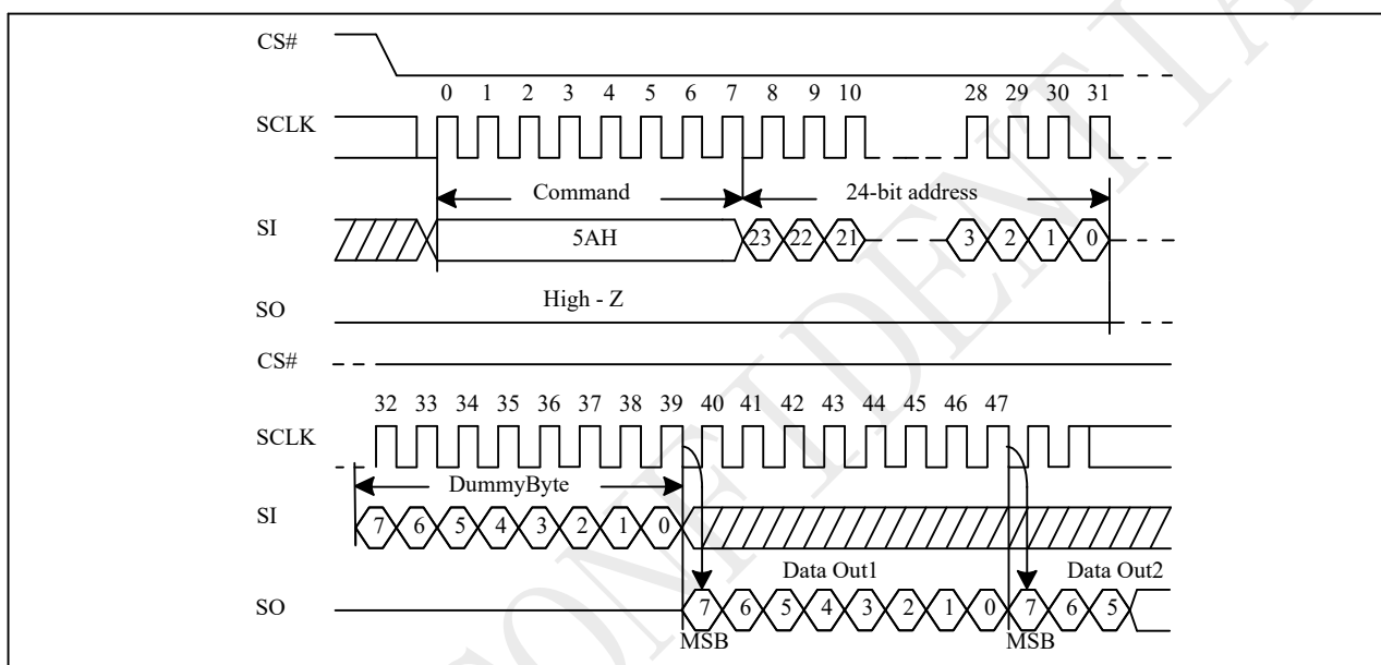
Figure 10-70 Read Serial Flash Discoverable Parameter (RDSFDP) Sequence (SPI)
