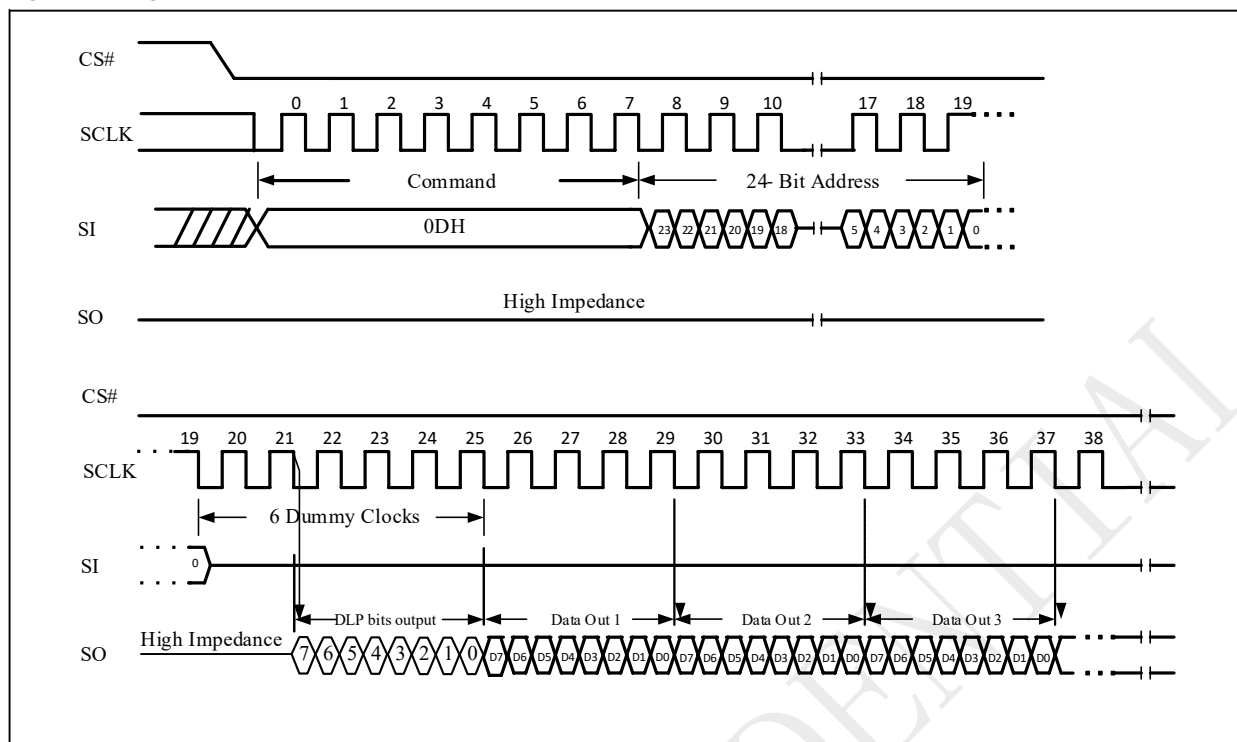
Figure 10-33g DTR 1IO Read with DLP bits output Sequence (SPI)
