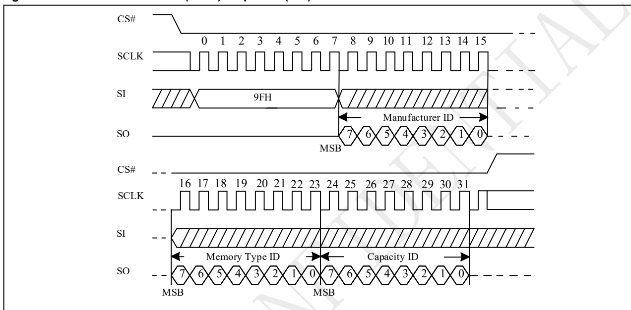
Figure 10-57a Read Identification (RDID) Sequence (QPI)
