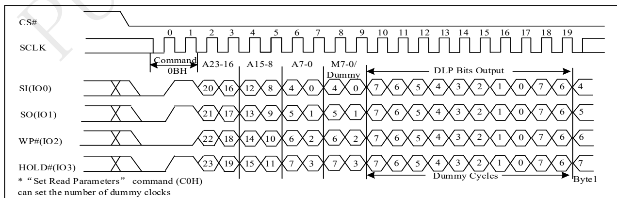
Figure 10-33a Fast Read with DLP bits output Sequence (QPI)
