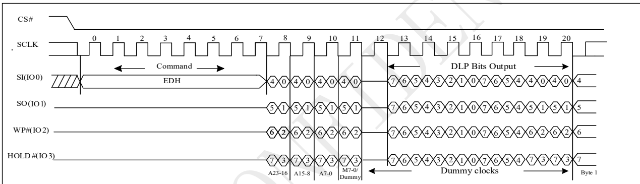
Figure 10-33j DTR 4IO Read with DLP bits output Sequence (SPI)
