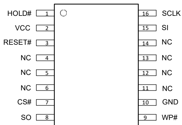
Figure 3-2 for SOP16 package
