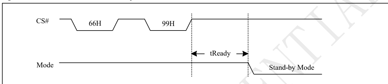
Figure 10-66 Software Reset Recovery
