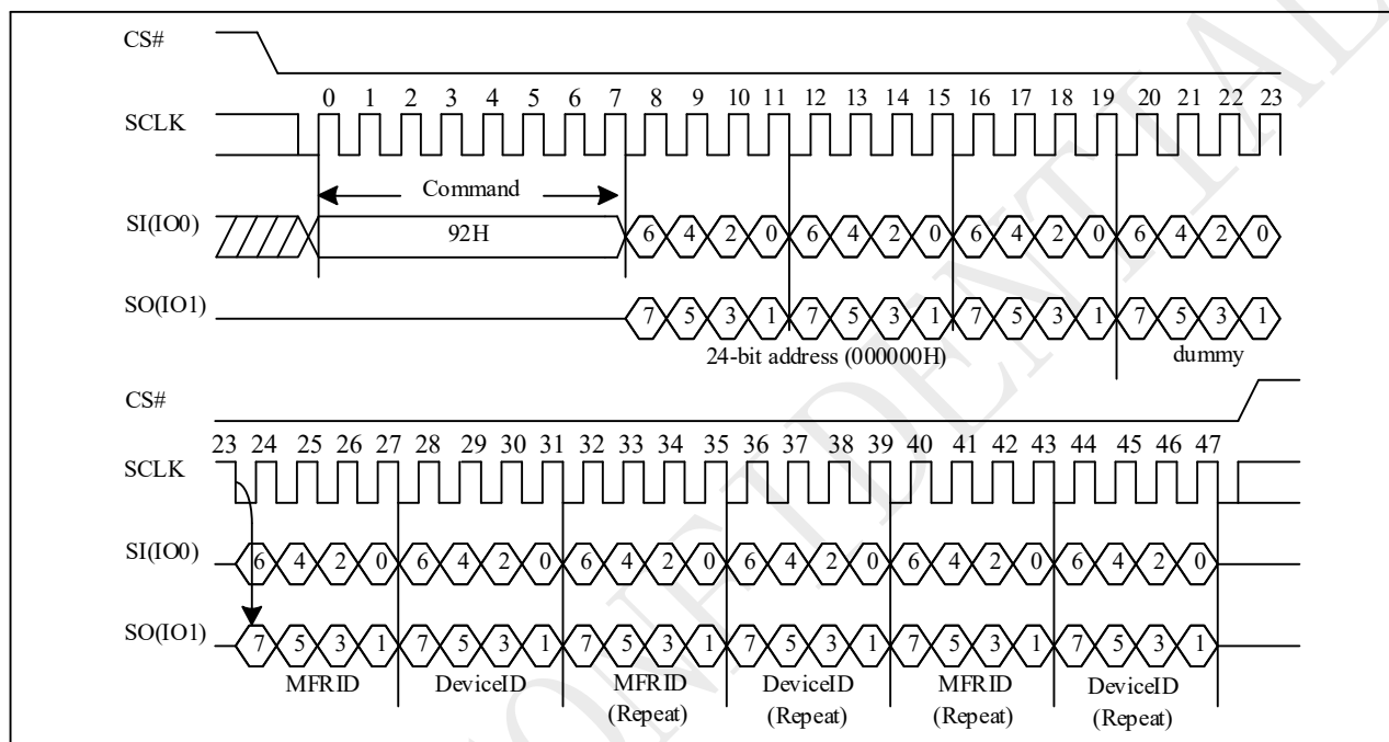
Figure 10-55 DUAL I/O Read Electronic Manufacturer & Device ID (DREMS) Sequence (SPI)
