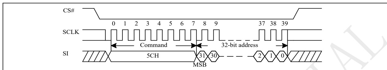
Figure 10-39 Block Erase 32K with 4-Byte Address (BE32K4B) Sequence (SPI)
