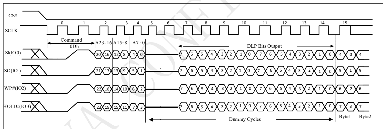
Figure 10-33i DTR 2IO Read with DLP bits output Sequence (SPI)
