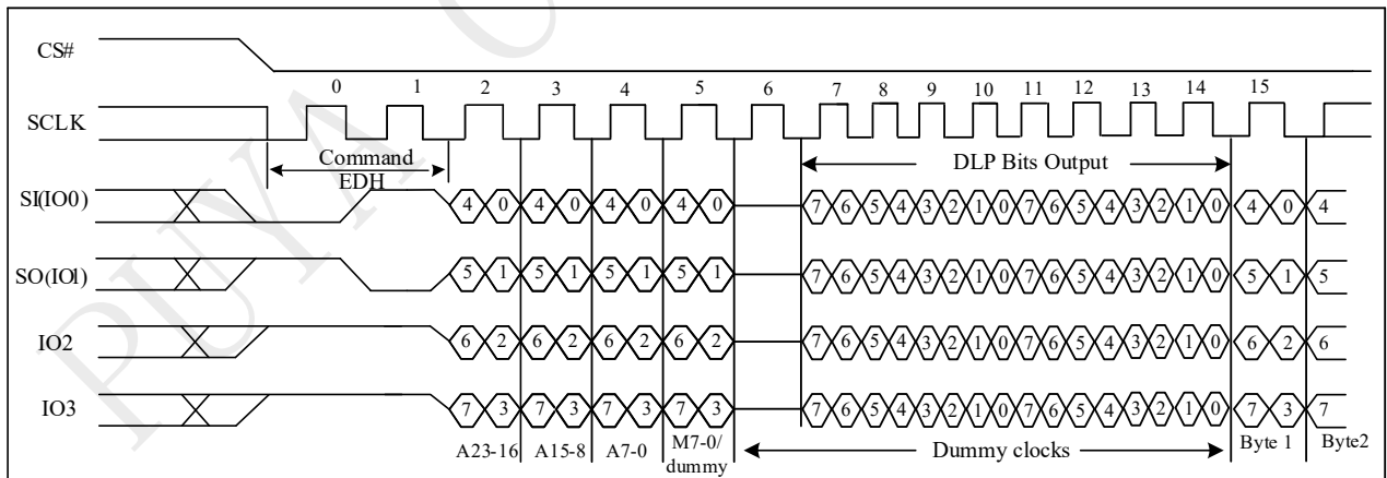
Figure 10-33k DTR 4IO Read with DLP bits output Sequence (QPI)
