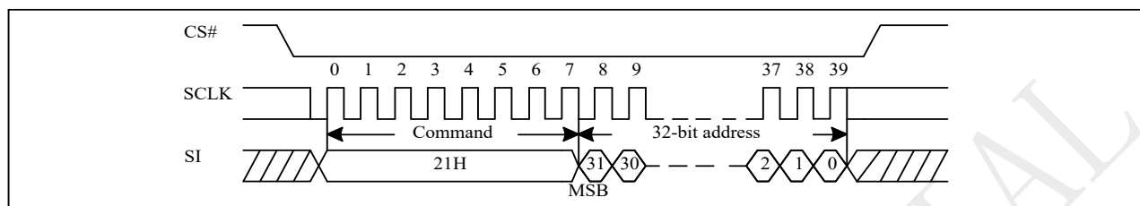
Figure 10-37 Sector Erase with 4-Byte Address Sequence (SPI)
